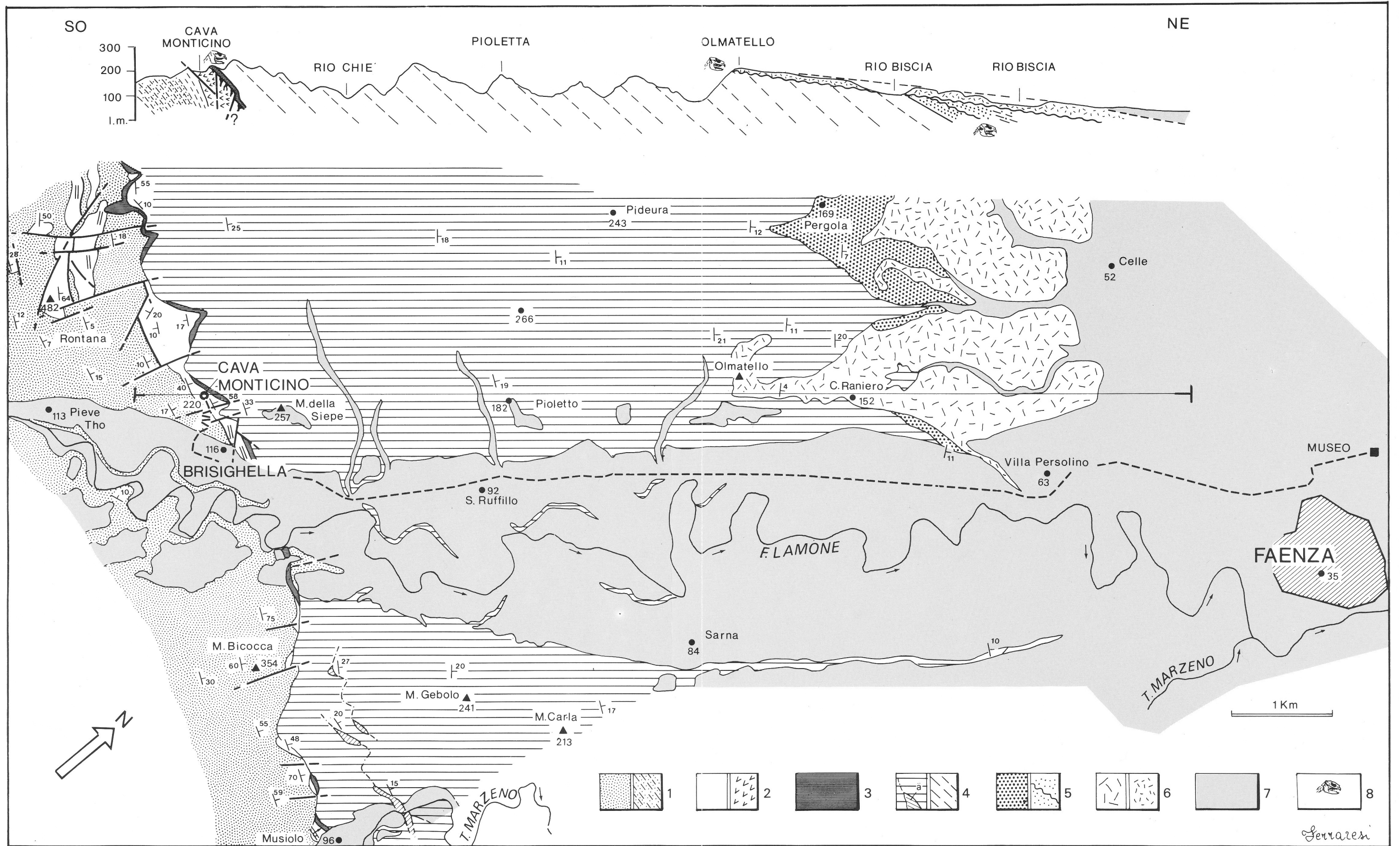
Geological map and cross section of the middle Lamone Valley showing location of the late Messinian Monticino fauna and of recent Pleistocene large mammal findings. 1, Marnosa-arenacea Fm.; 2, Gessoso-solfifera Fm.; 3, Colombacci Fm.; 4, Argille Azzurre Fm. (a «Spungone» member); 5, «Sabbie gialle» fm.; 6, Olmatello Fm.; 7, Alluvial terraces; 8, faunal localities.
